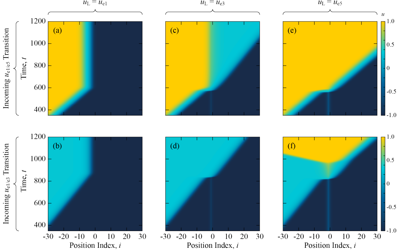
FIG. 3. Transition Wave Stabilization and Conversion. Spatio-temporal evolution of u_{e1/e5} - and u_{e1/e3} -mode transition waves in the lattice with prescribed u_L = \{u_{e1}, u_{e3}, u_{e5}\} , demonstrating wave stabilization and conversion according to the stated criteria in the text.
